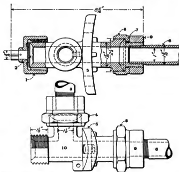
Figs. 3036-3037. Blower Valve Lever Stud.
